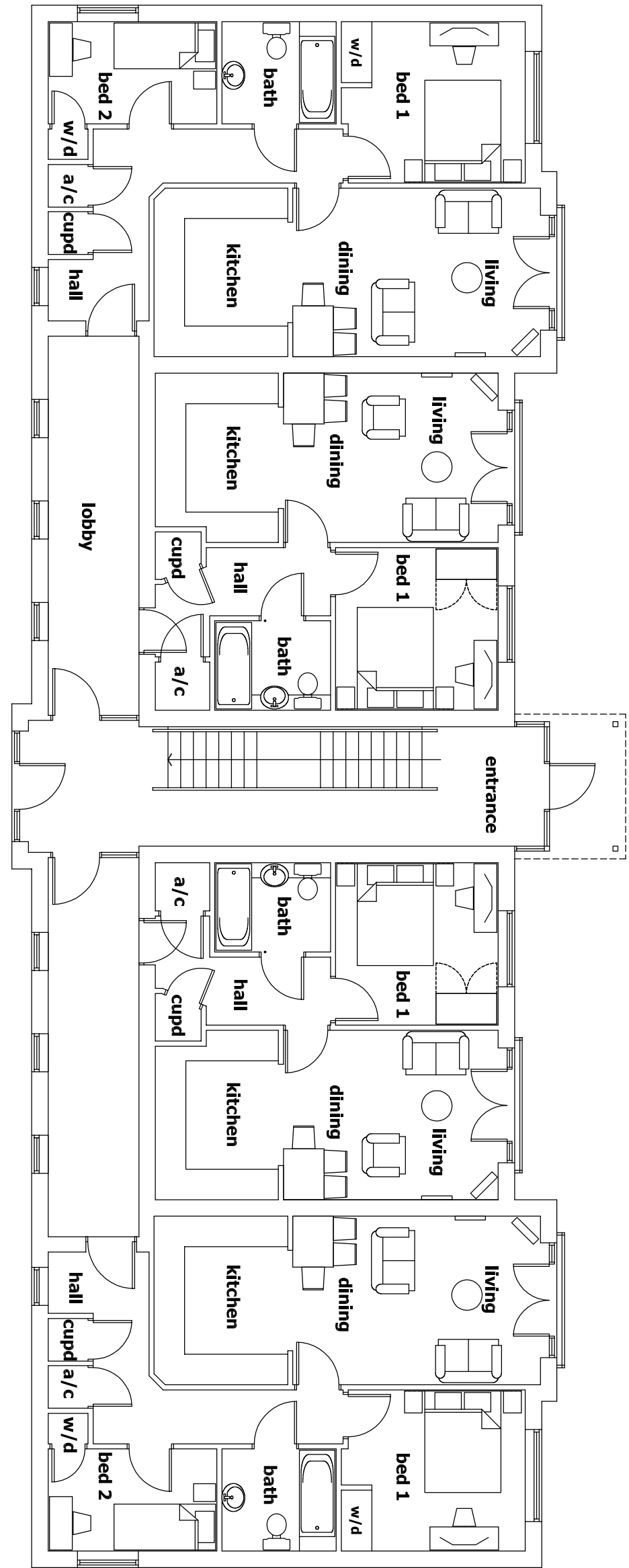
ground/first floor plan
