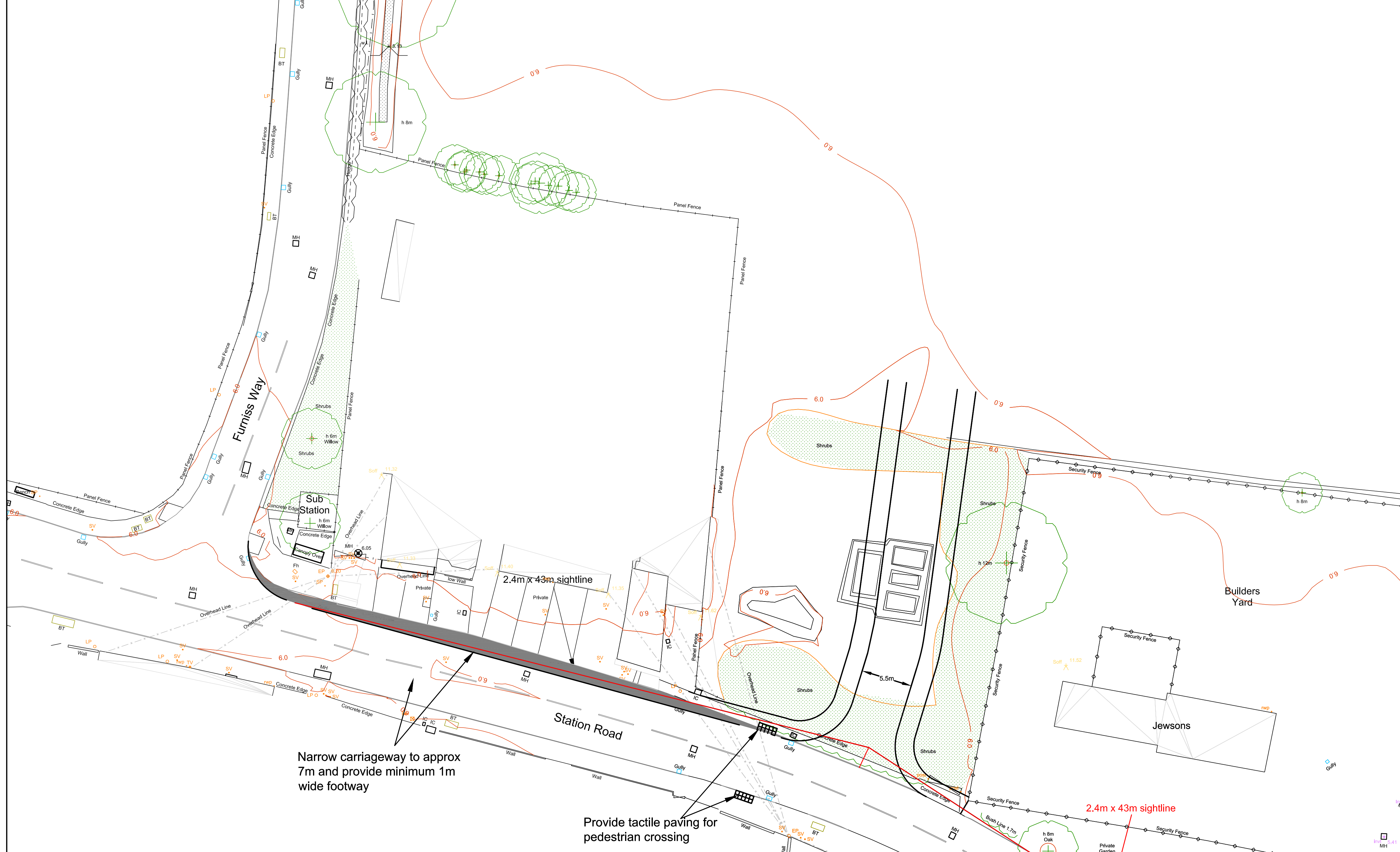
PROPOSED FOOTWAY IMPROVEMENTS
