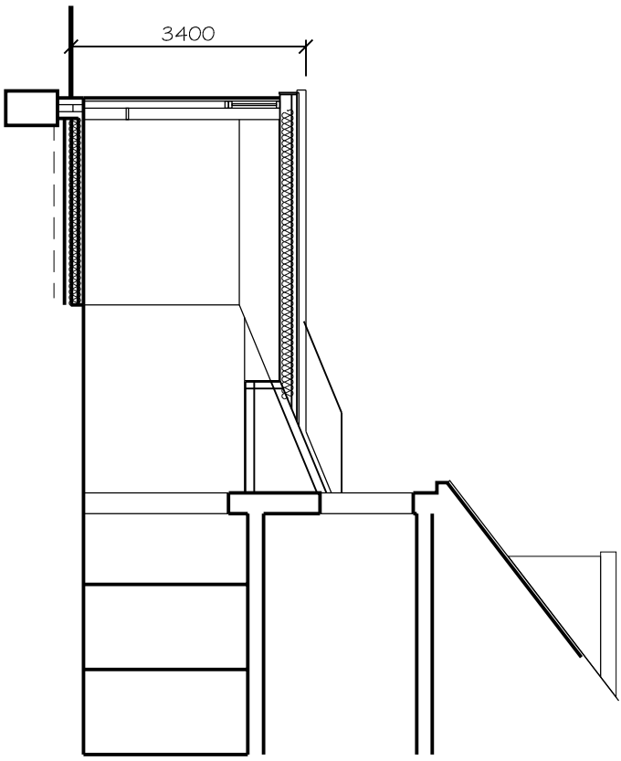
Section AA
