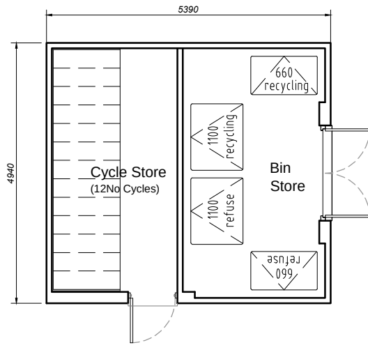
Floor Plan Flat Blocks B & E
