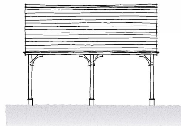
REAR ELEVATION
