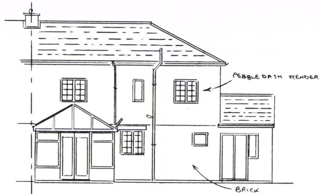
REAR ELEVATION (EAST)
