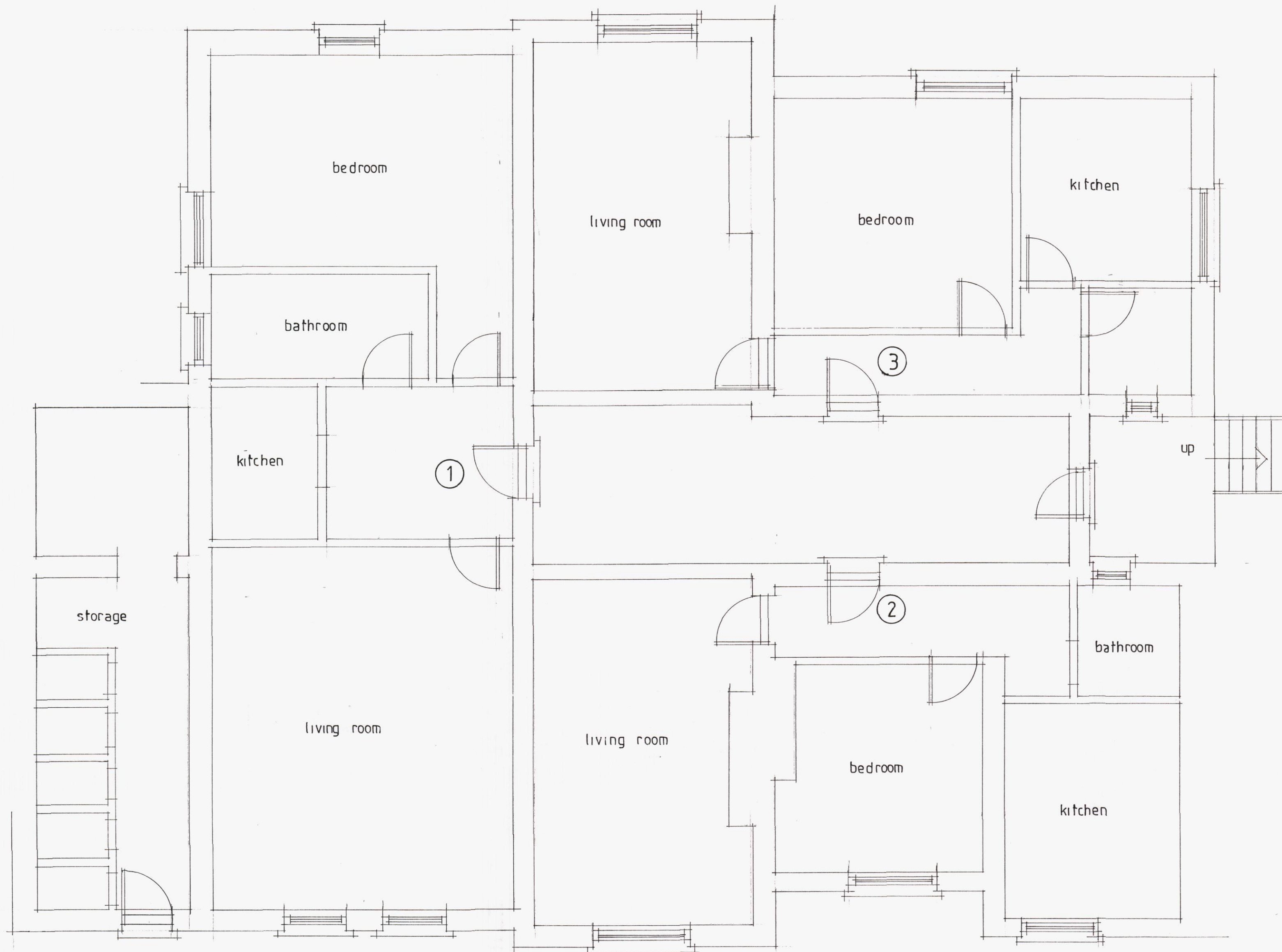
Existing Basement Plan
