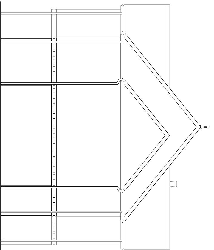
Side Elevation 1:100
