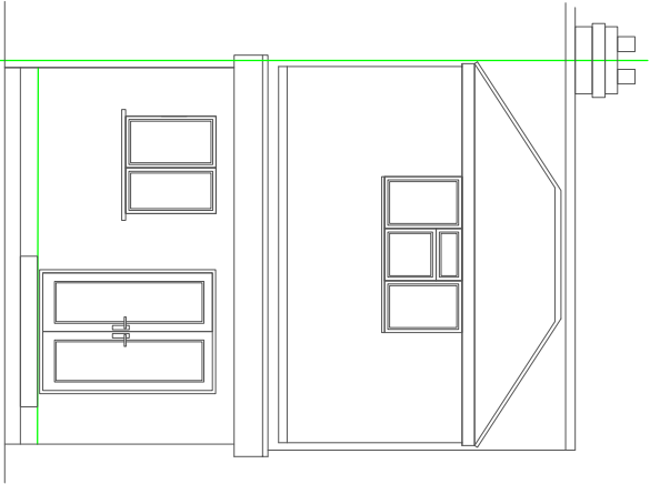
EXISTING REAR ELEVATION (UNDER PD)
