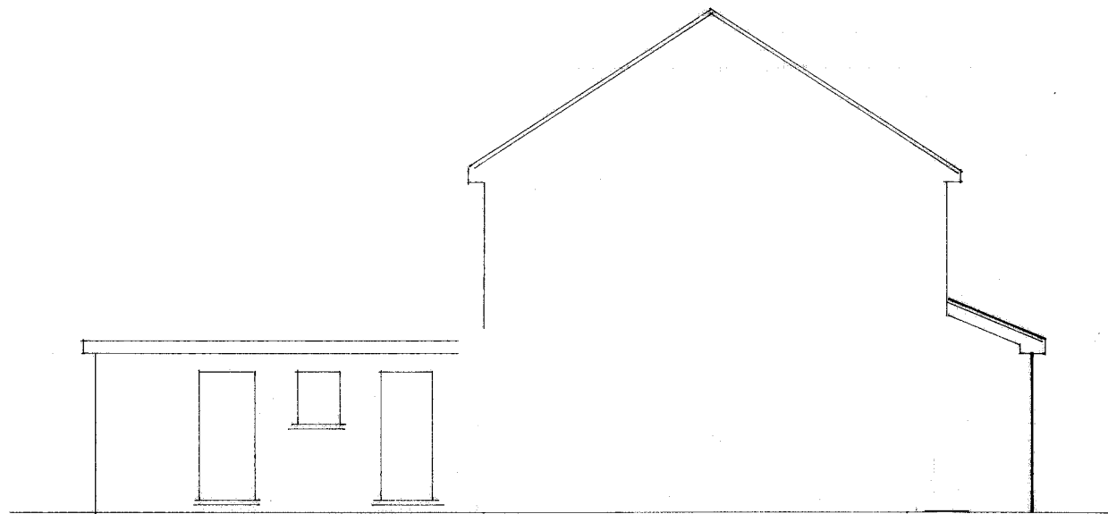
Proposed West/Side Elevation
