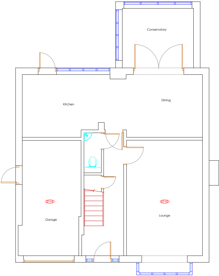
Proposed Ground Floor (No change)
