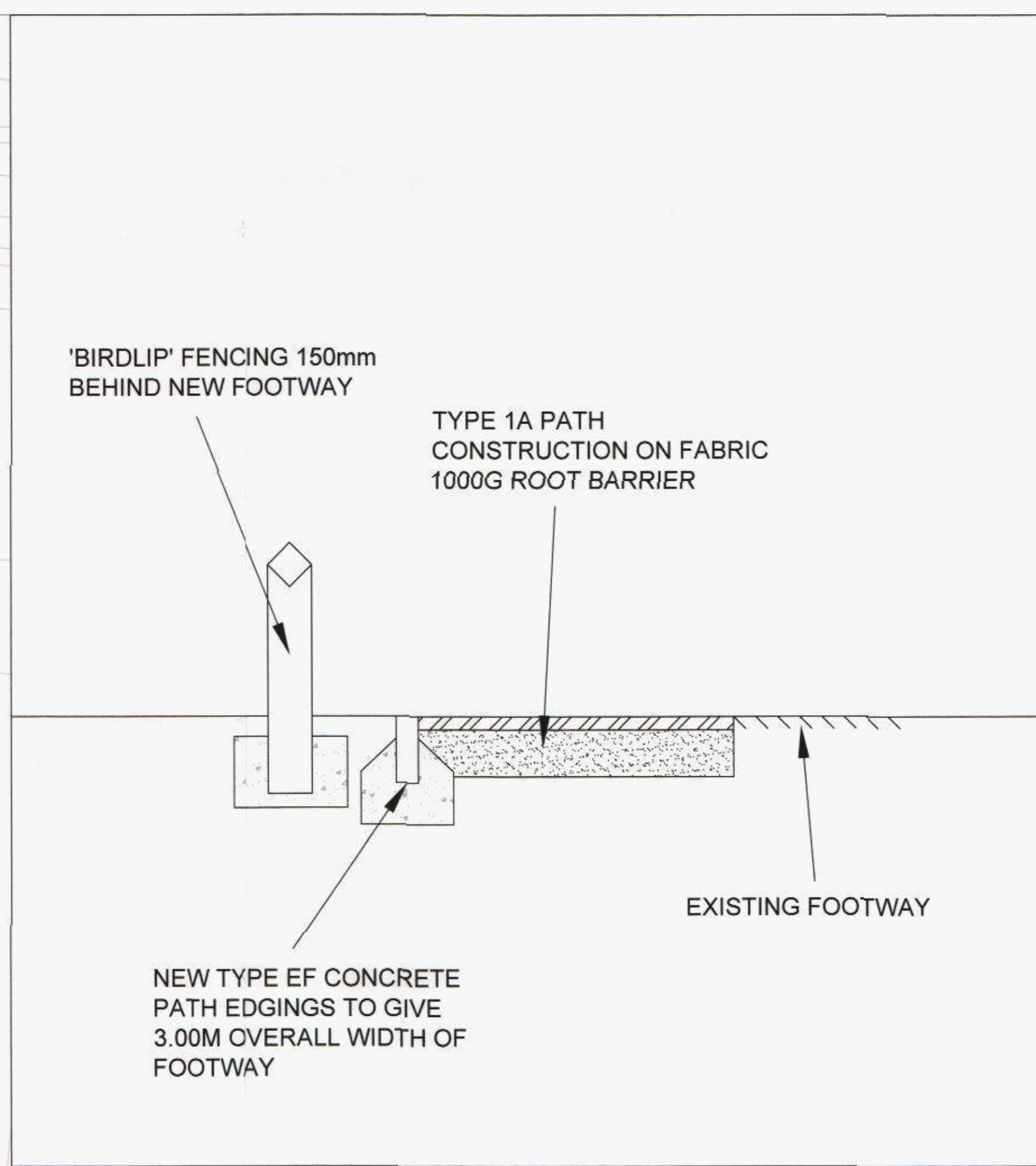
DETAIL OF EXTENDED PATH AND 'BIRDIP' FENCING NOT TO SCALE
