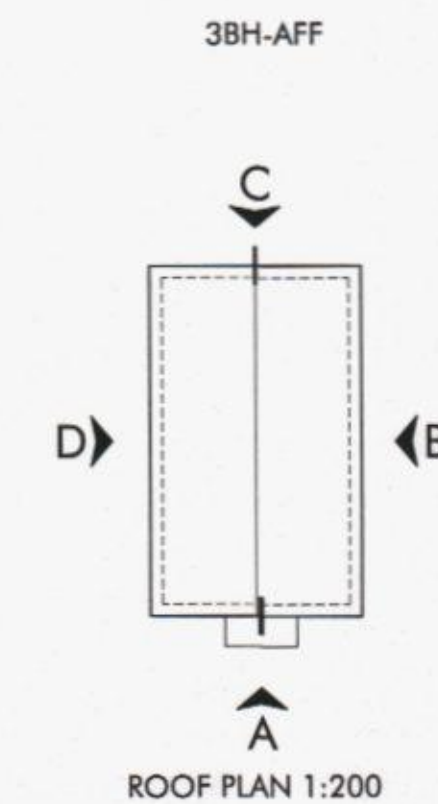
ROOF PLAN 1:200
