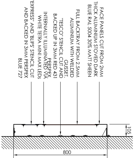
Section scale 1:20 Fascia Sign
