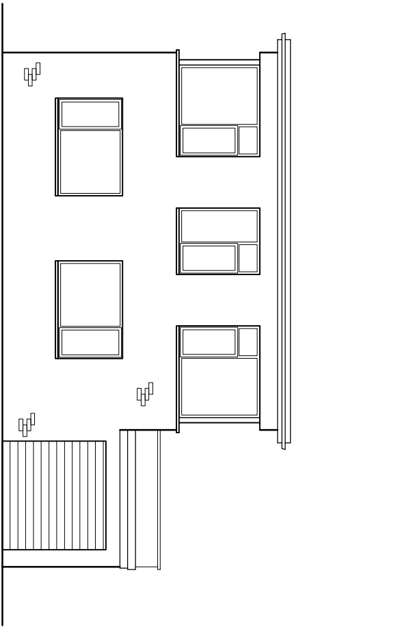
Front (east)
