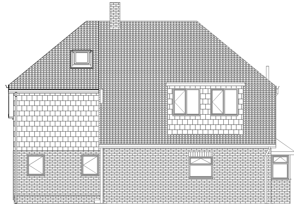
ELEVATION SOUTH EAST 1 : 100
