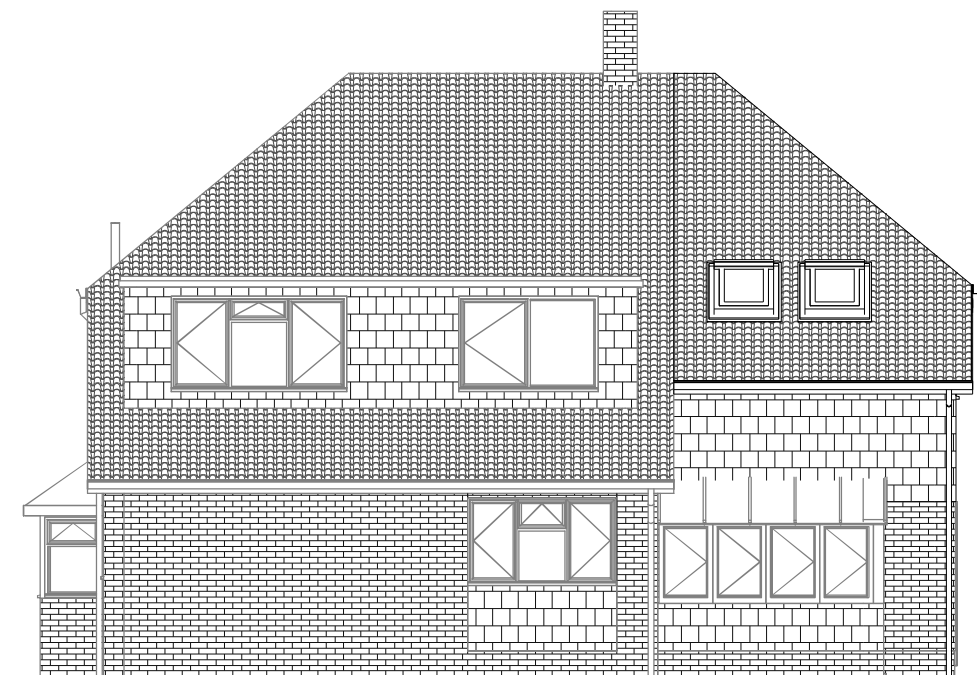
ELEVATION NORTH WEST 1 : 100
