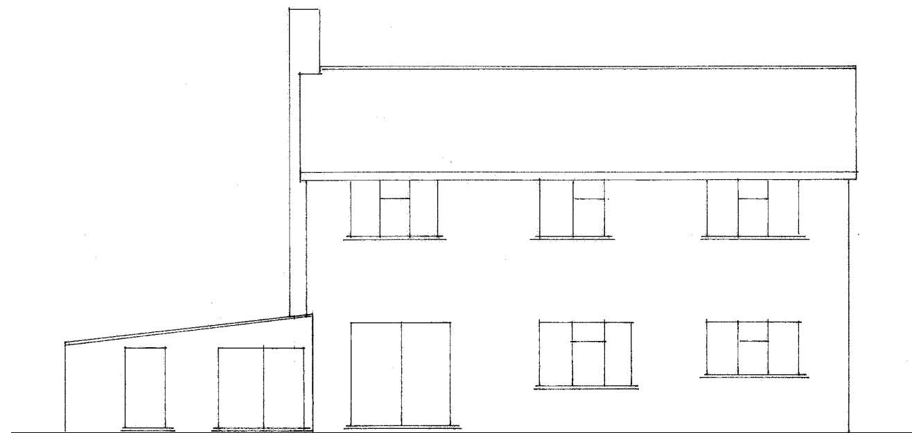
Existing SE/Rear Elevation
