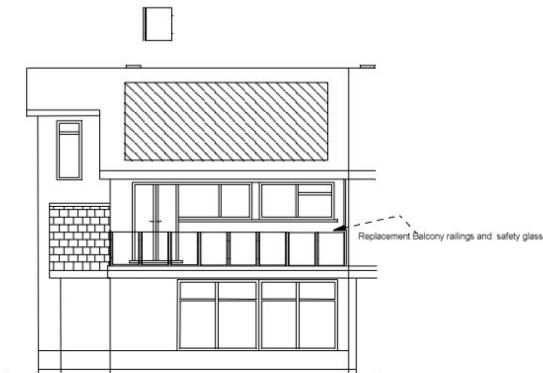
South Elevation
