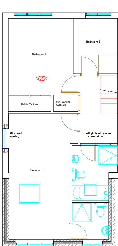
Proposed First Floor
