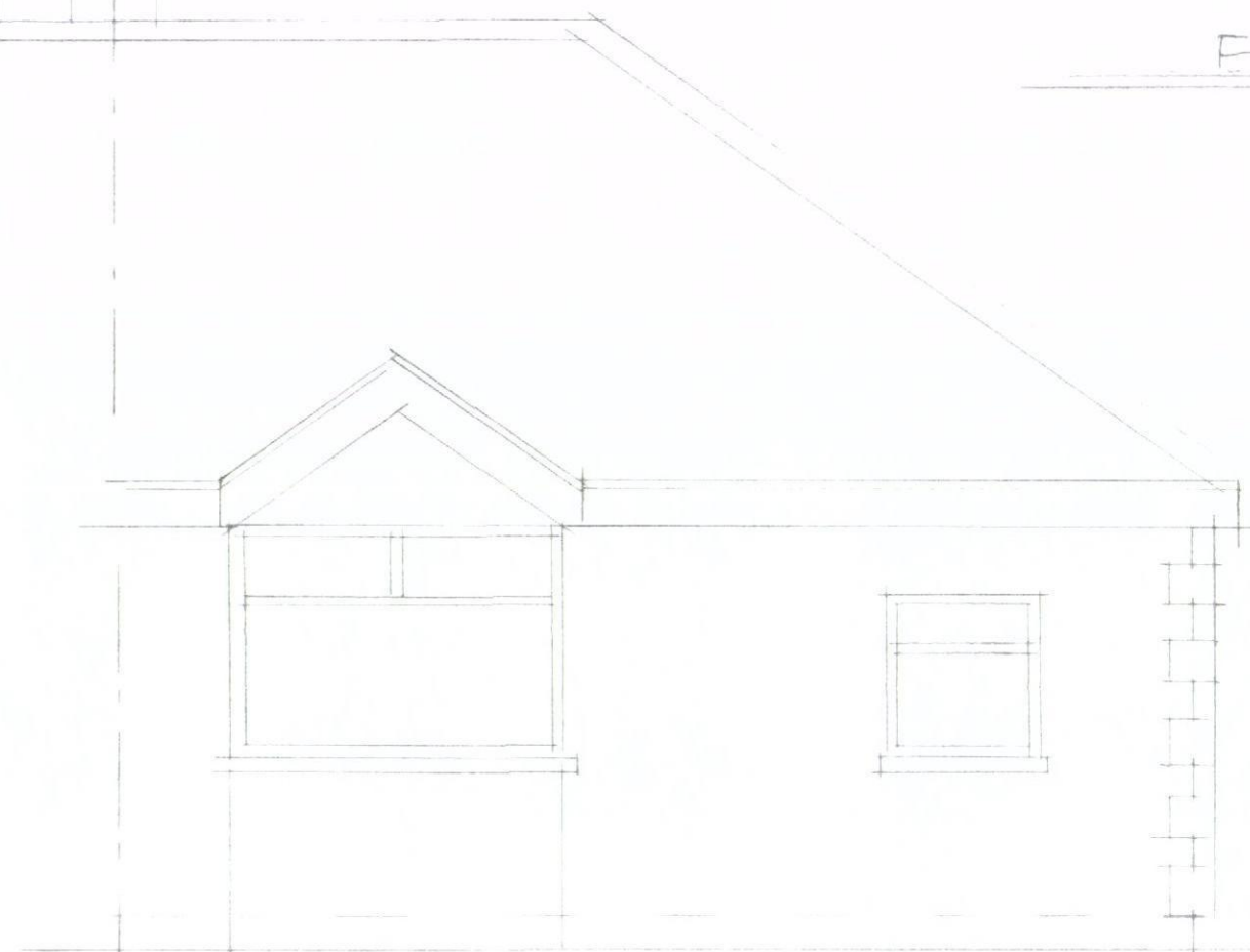
EXG FRONT ELEVATION
