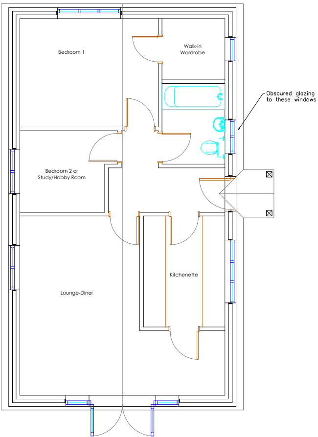
PROPOSED FLOOR PLANS
