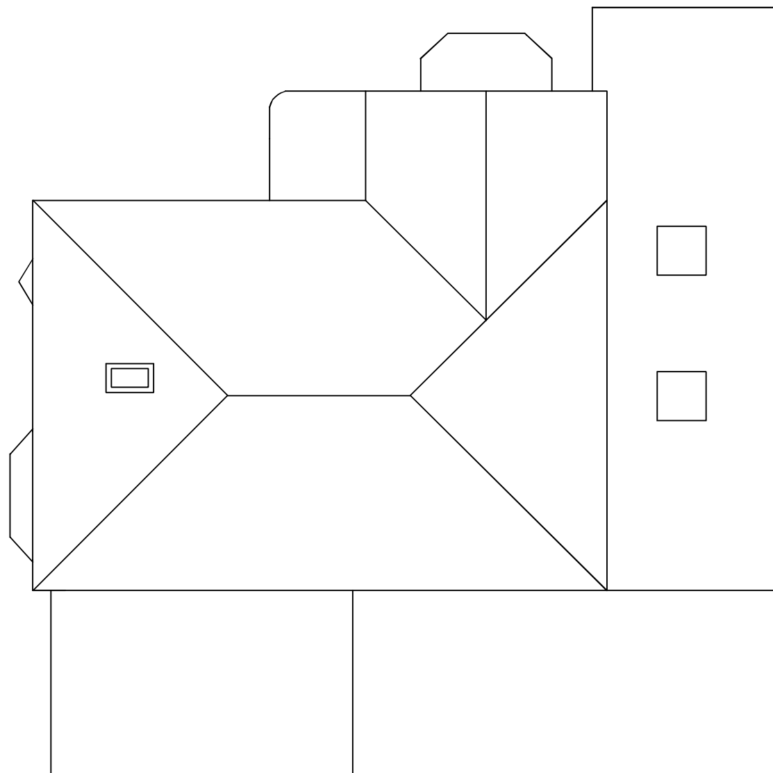
Proposed Roof Plan Scale 1/100@A3
