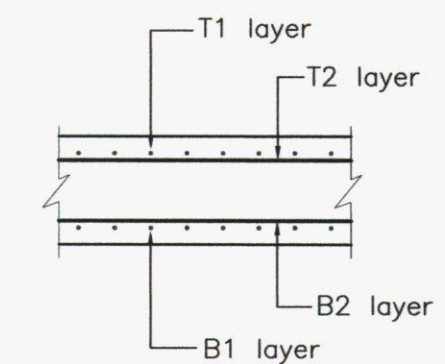
Reinforcement layering (1:20)
