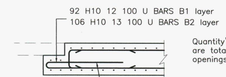
Typical edge detail at access holes (1:20)
