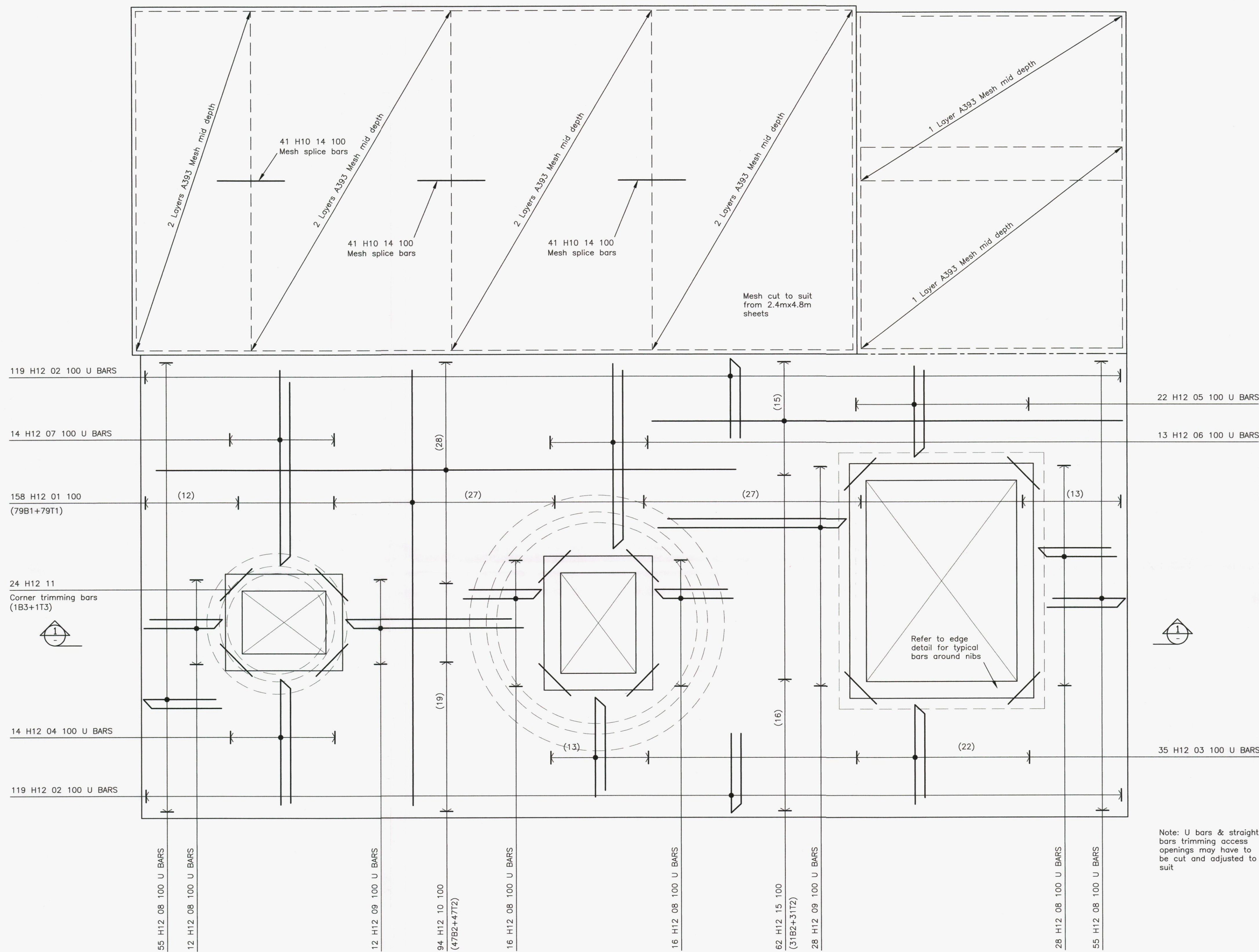
RC plan at compound level (1:25)
