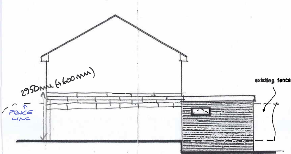
East Elevation. EXISTING 2004
