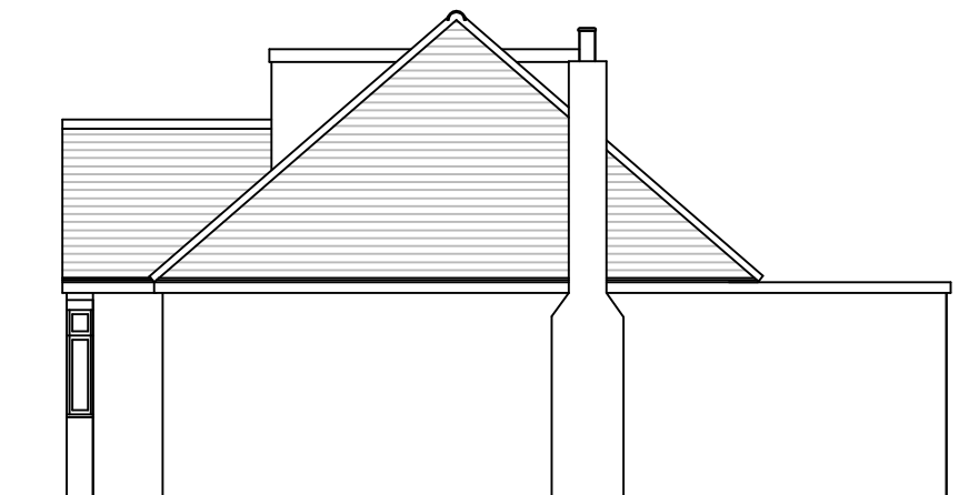
Existing RHS Elevation Scale 1/100@A3
