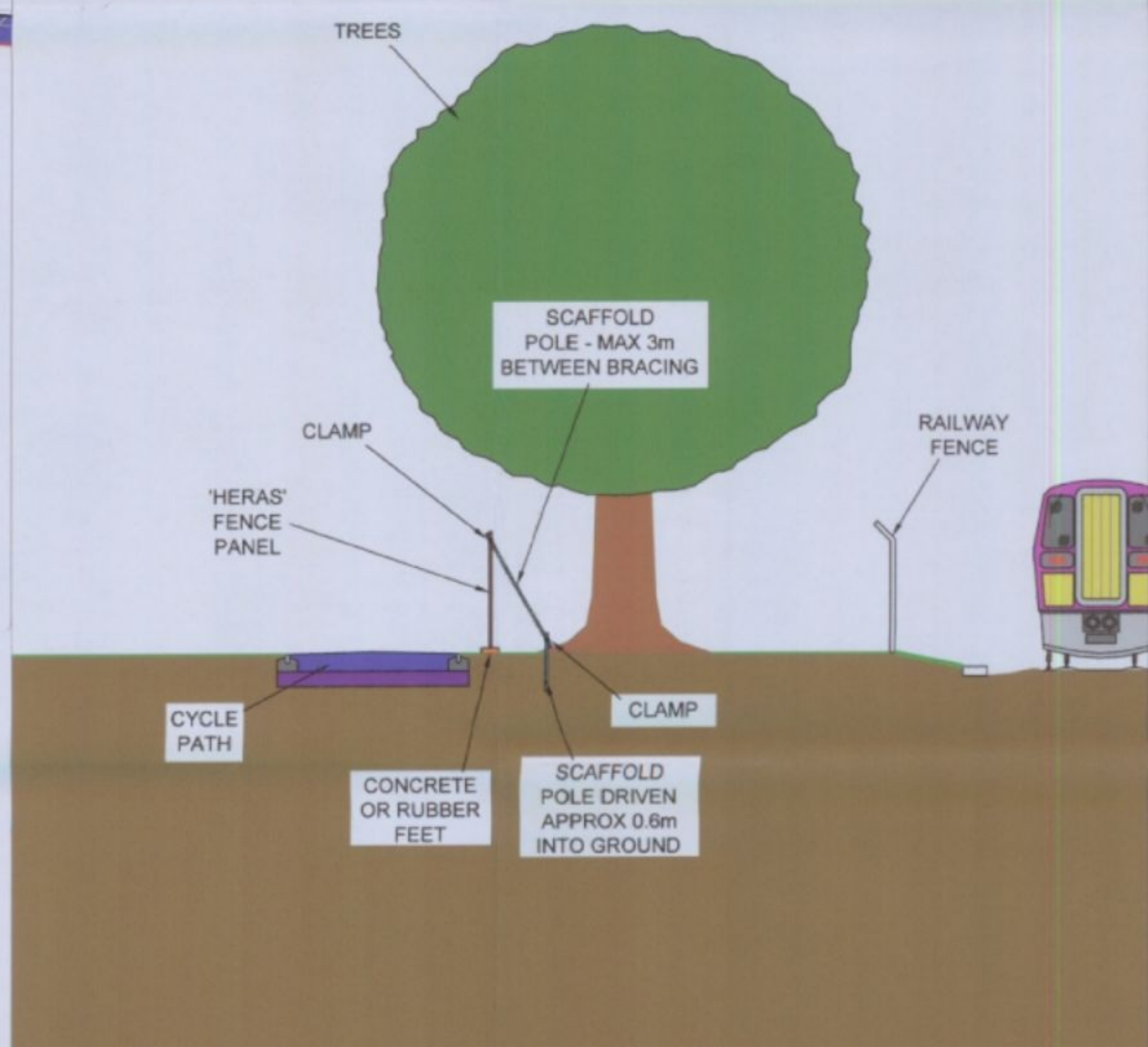
DETAIL OF TEMPORARY FENCING AROUND TREE DURING PATH CONSTRUCTION NOT TO SCALE
