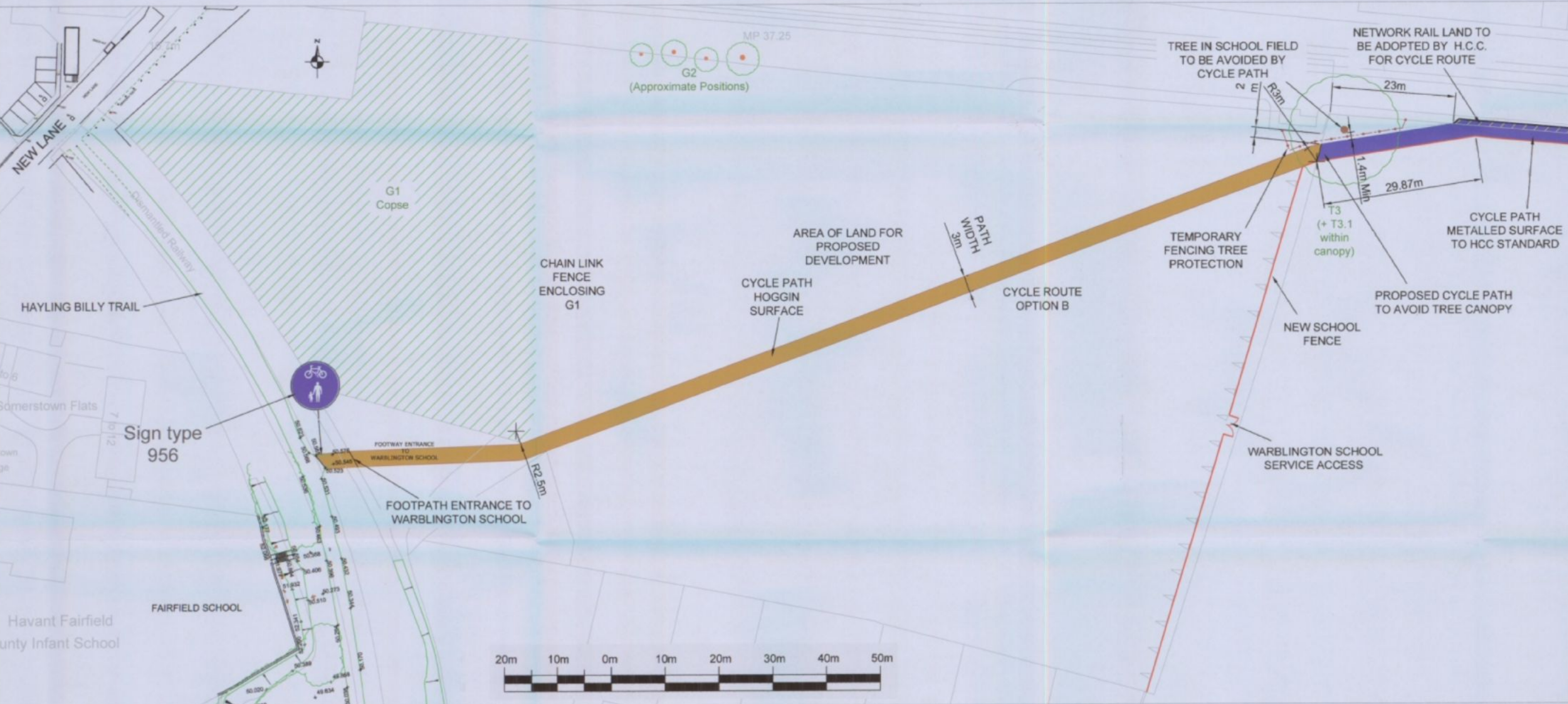
DETAIL 1 SCALE 1:500
