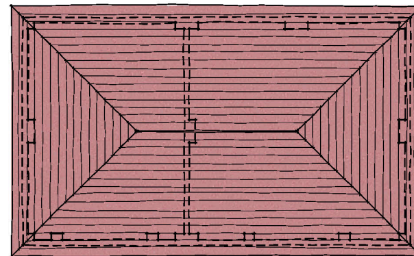
ROOF PLAN
