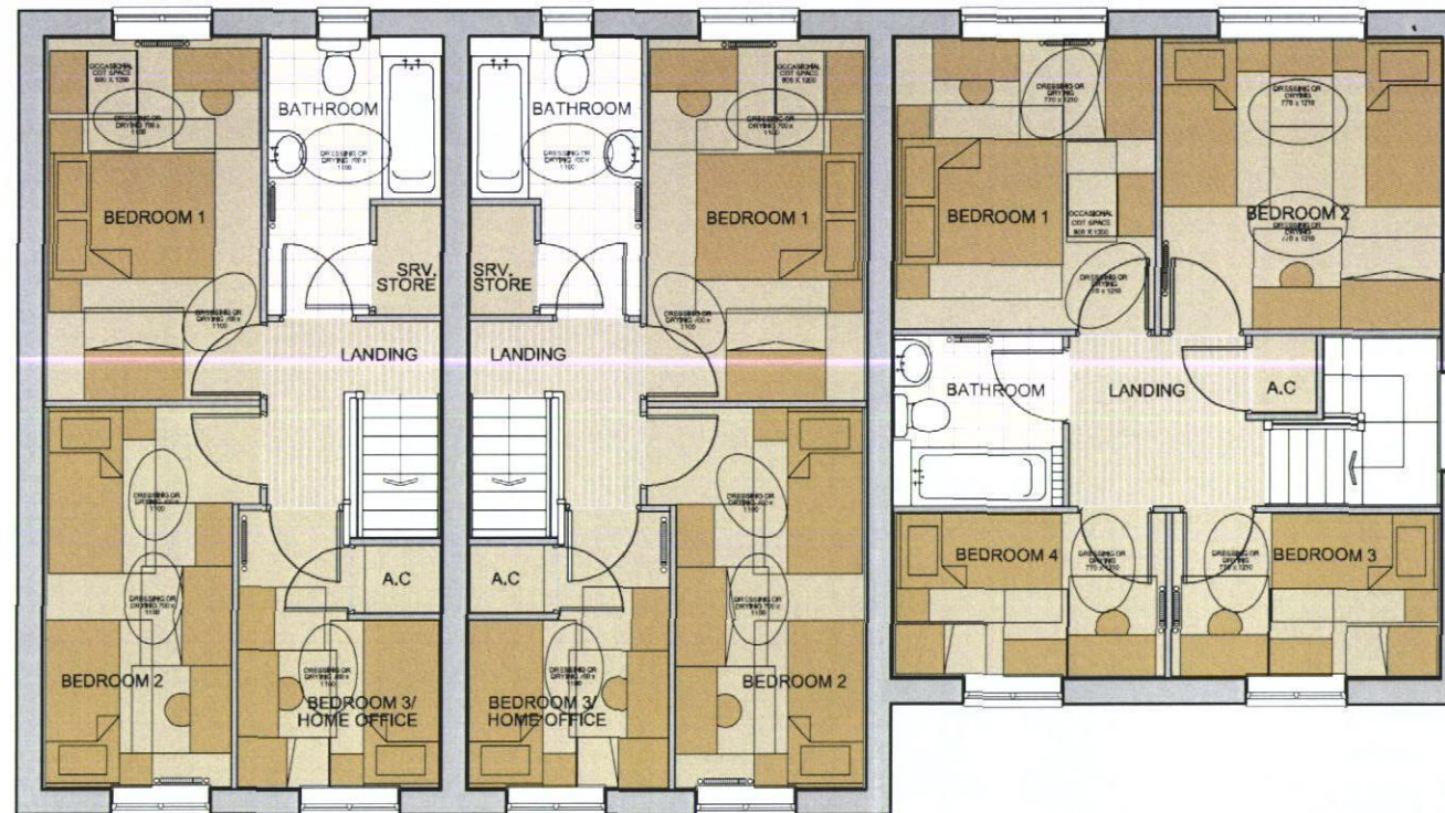
FIRST FLOOR
