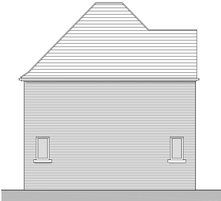
Proposed Side Elevation - South
