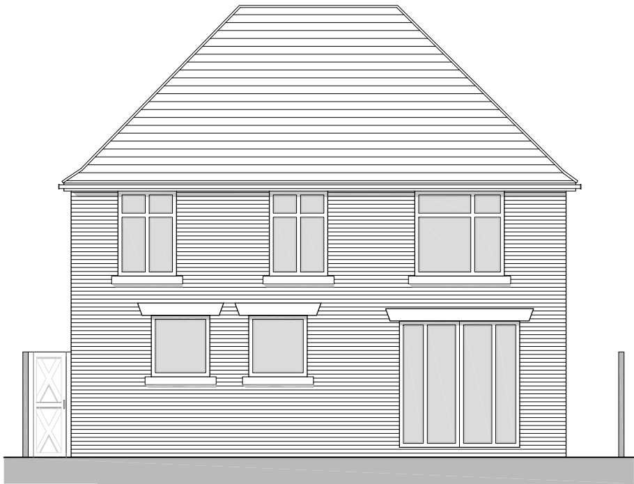
Proposed Front Elevation - West
