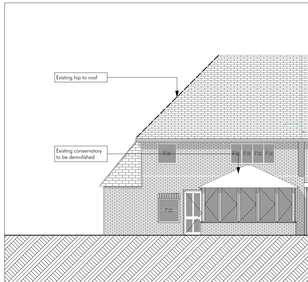
N North Elevation Existing 1:100
