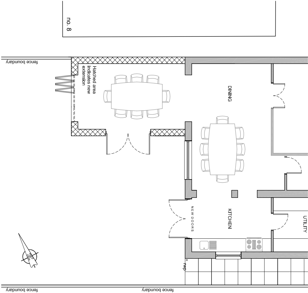
PART GROUND FLOOR PLAN
