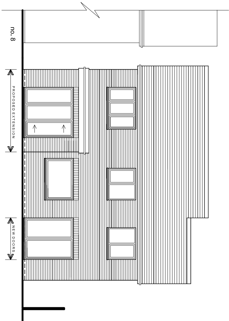
REAR ELEVATION
