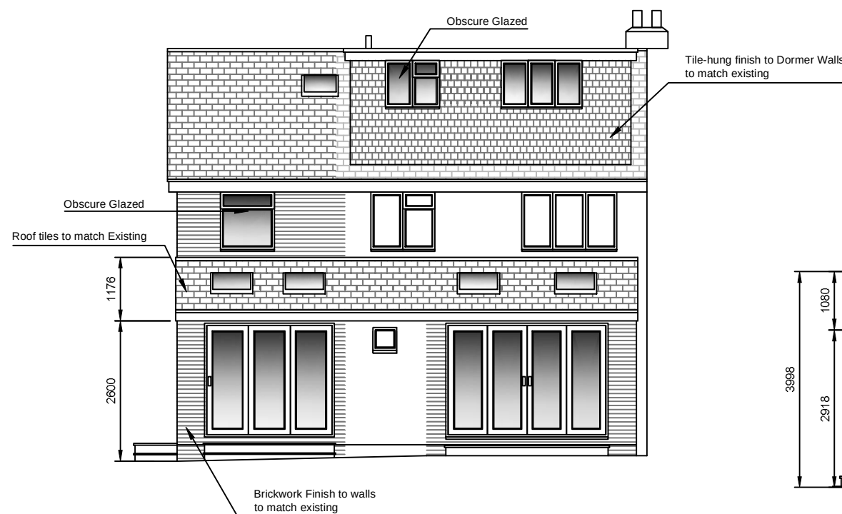
Rear Elevation
