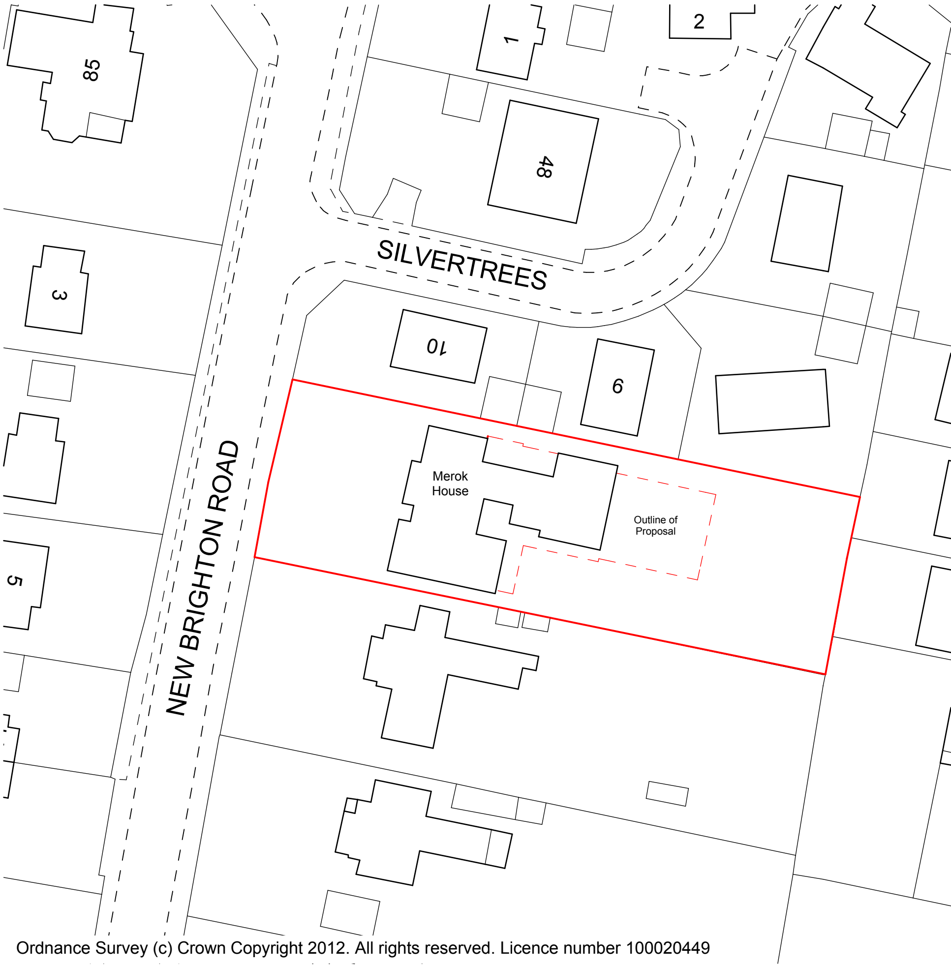
OS Plan Block 1:500
