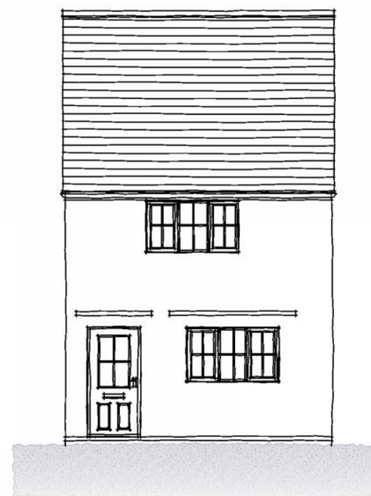
REAR ELEVATION
