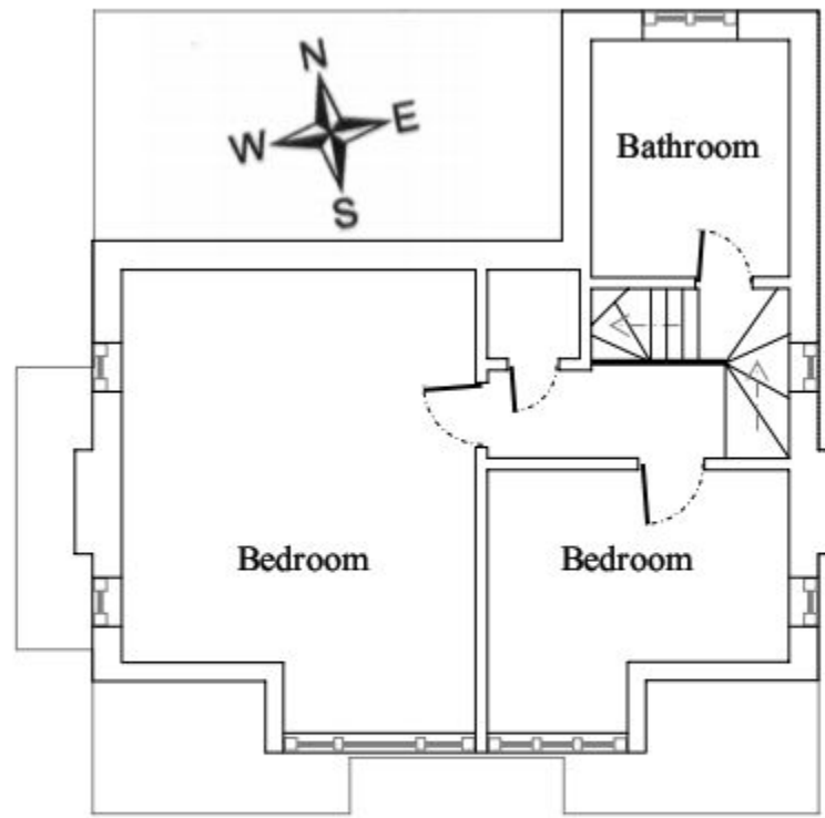
Existing Upstairs Floor Plan
