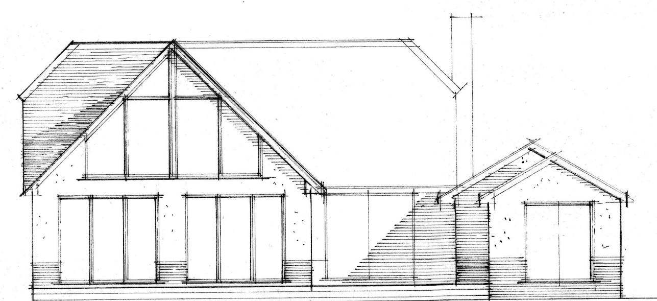
proposed rear
