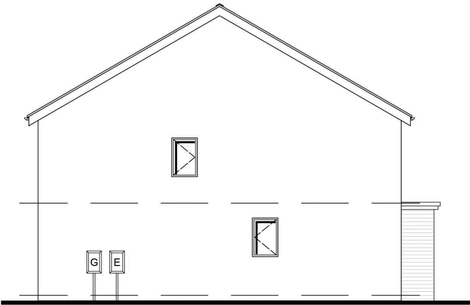
SIDE ELEVATION
