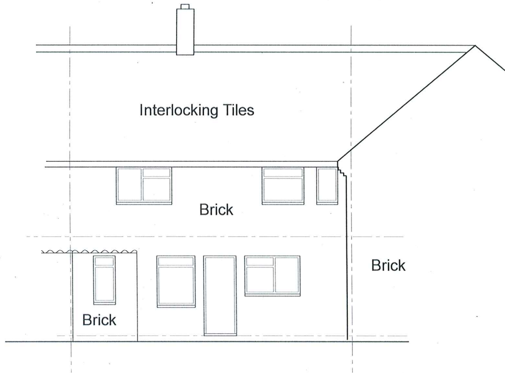
Existing Rear - South Elevation
