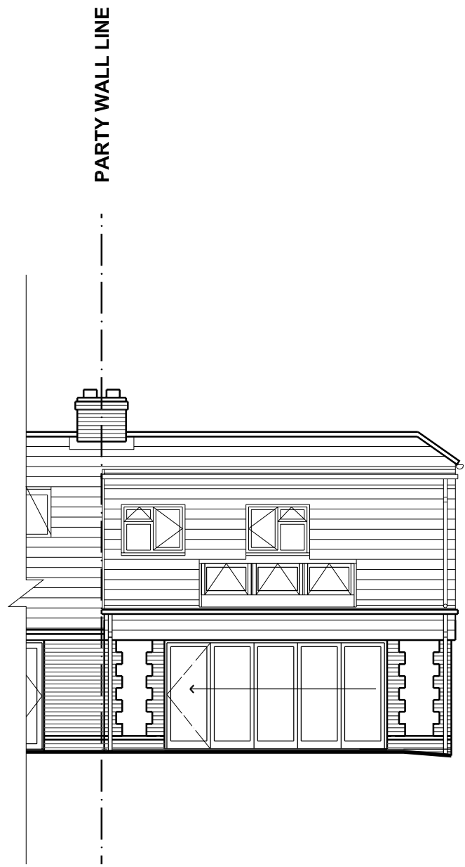
REAR ELEVATION
