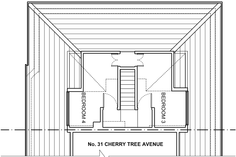
FIRST FLOOR
