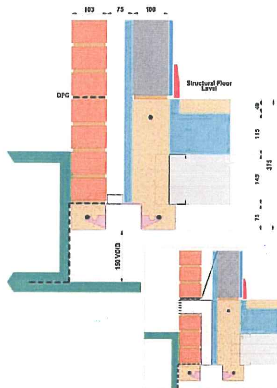
Fig 1: Detail at ventilation position
