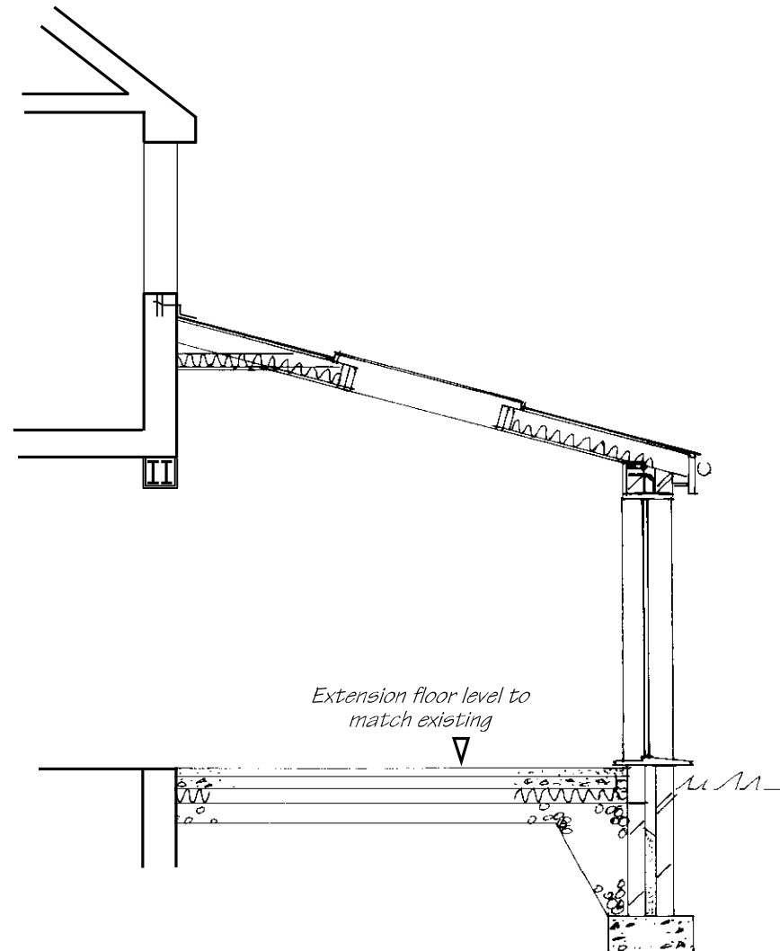
Cross-Section
