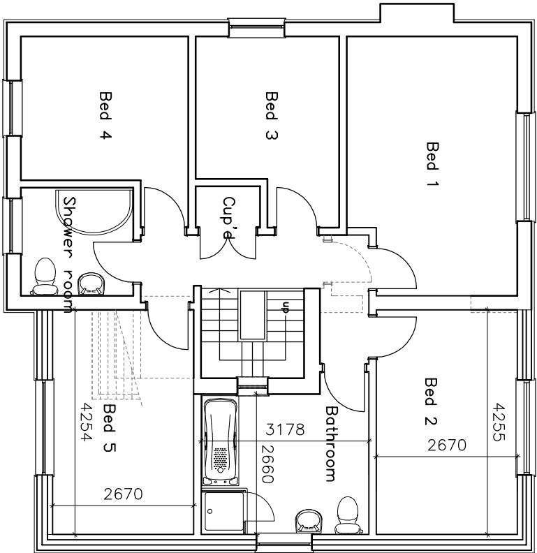
1st Floor Plan as proposed
