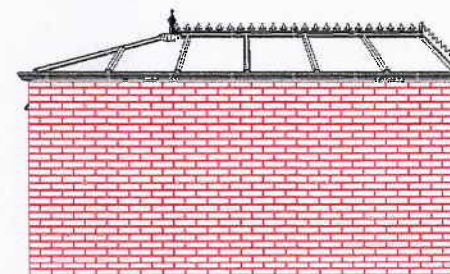
RIGHT VIEW
