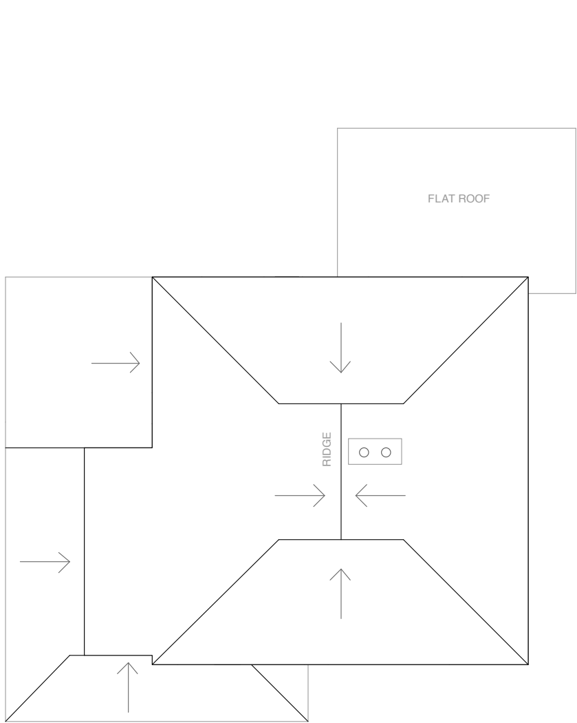
Existing Roof Plan at 1:100 scale
