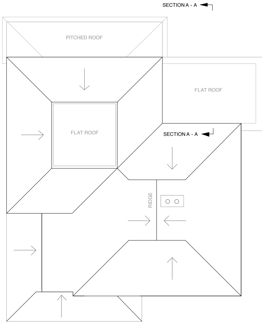
Proposed Roof Plan at 1:100 scale
