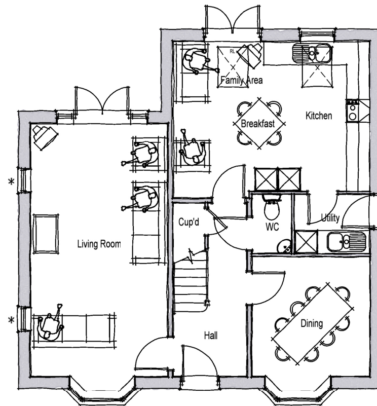
GROUND FLOOR PLAN * PLOT 18 ONLY
