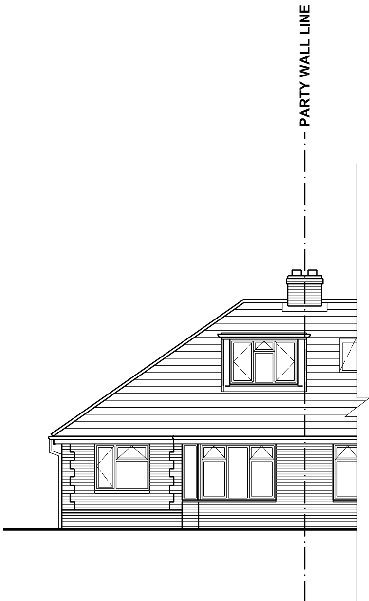
FRONT ELEVATION
