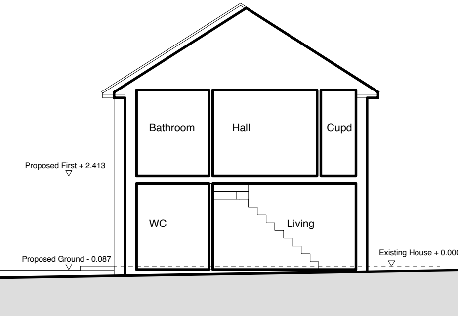
PROPOSED SECTION 1:100
