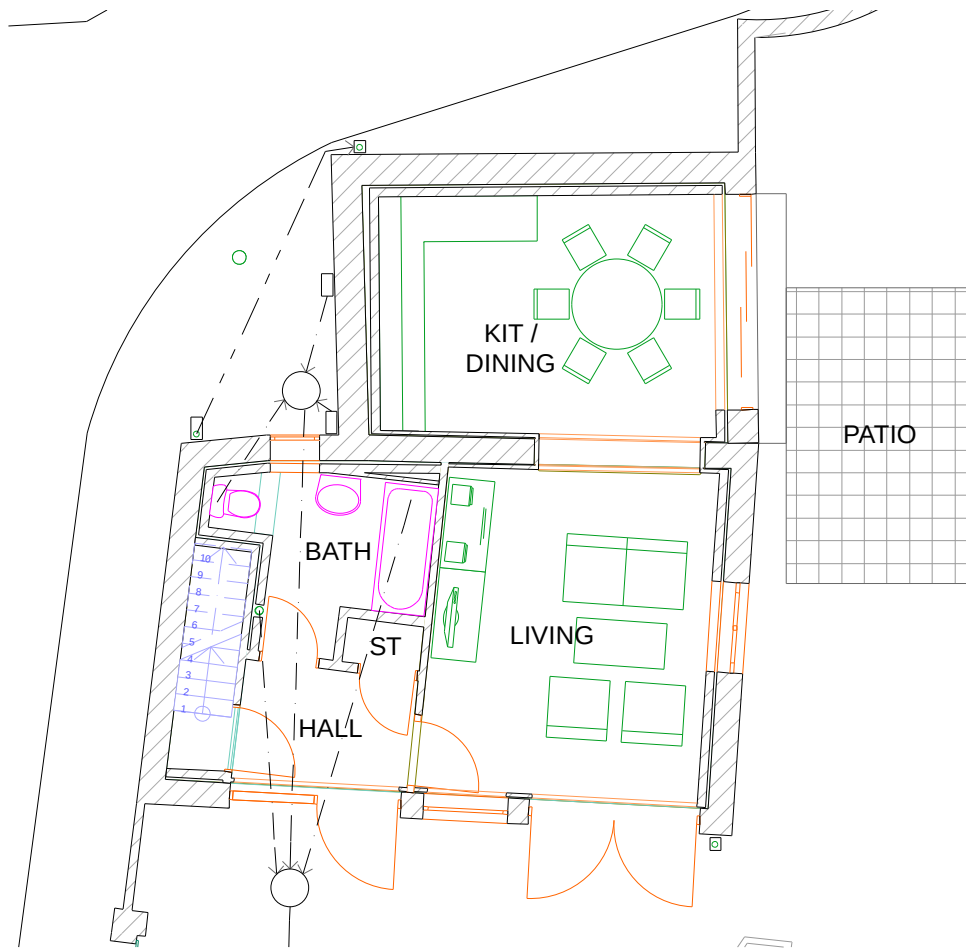
GROUND FLOOR PLAN: AS PROPOSED
