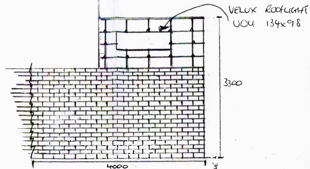
WEST ELEVATION 1:50
