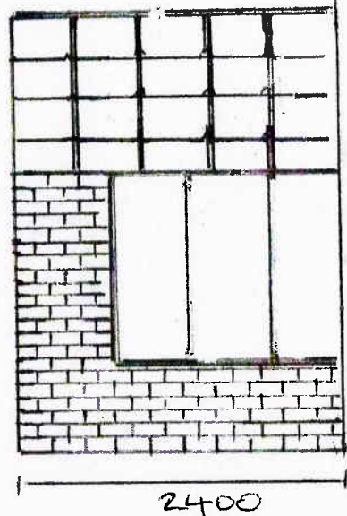
EAST ELEVATION 1:50
